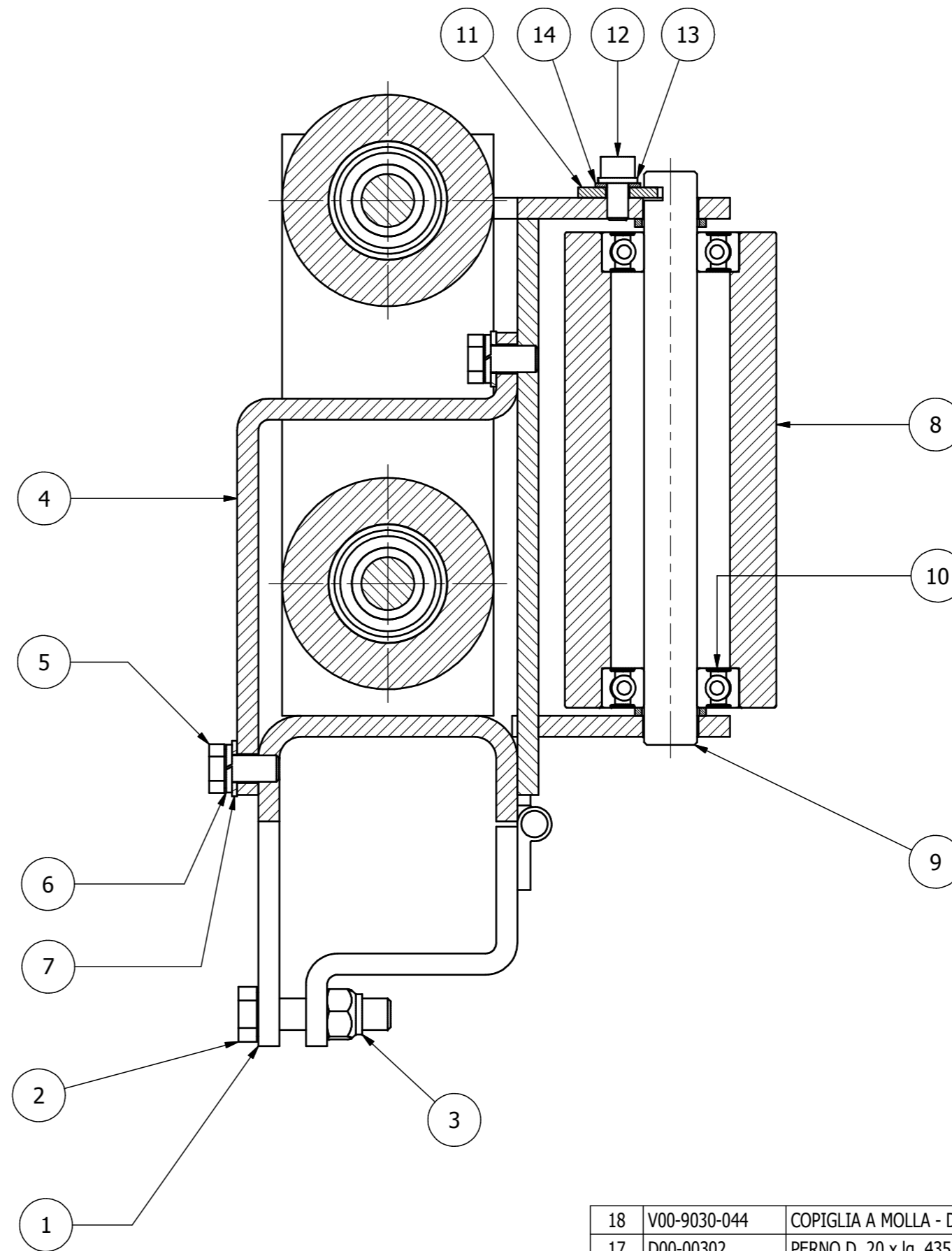
F-F (1:2)
