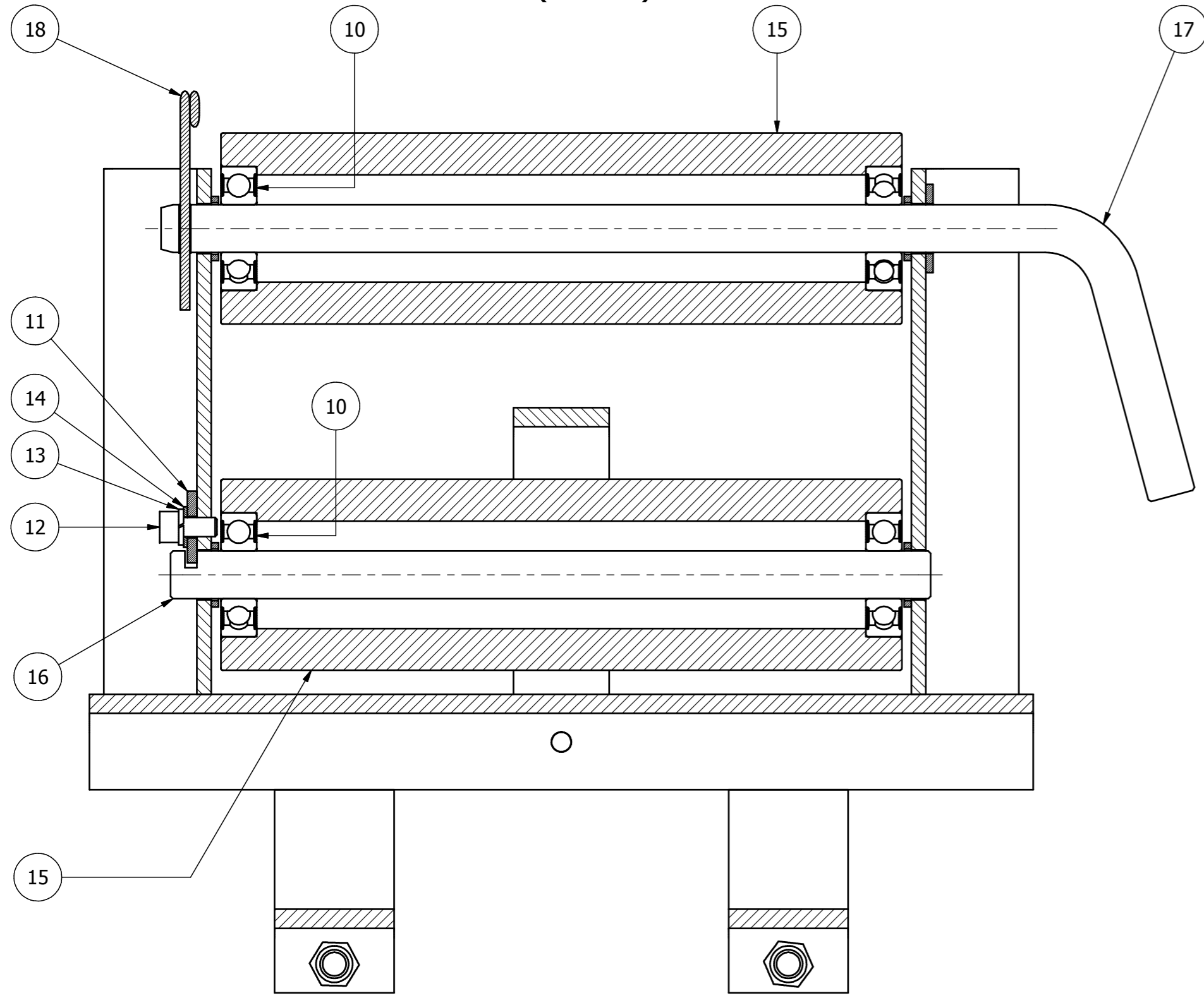
E-E (1:2)
