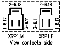
View contacts side
